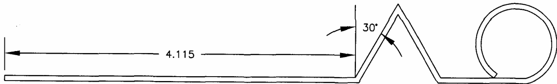
Dip Stick FIG. 1
